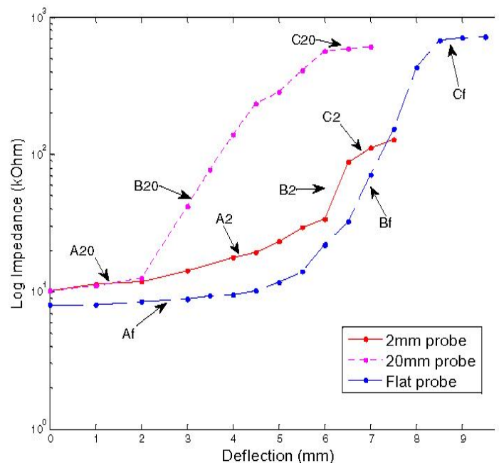
Figure 8: Log impedance (1-1000 kΩ) versus static deflection of skin applied by three probes with different curvatures. Three distinct operating regions (labeled A, B and C) are present for each curve and discussed in text.
