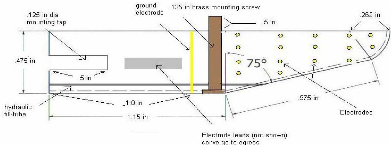
Figure 2. Mechanical Drawing of Second Prototype
