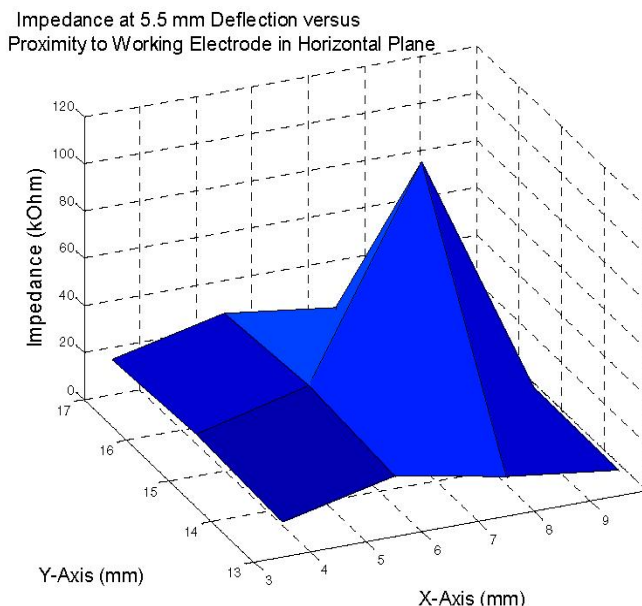
Figure 10: Impedance as a function of center of pressure with respect to the electrode location.
