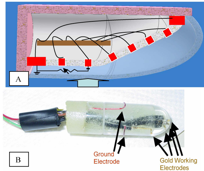
Figure 1: A) Mechanical drawing of the biomimetic tactile sensor showing a rigid core shaped like the distal phalanx (white) with an internal, sealed compartment for electronics (brown) connected to sensing electrodes (red) in contact with a weakly conductive fluid under a viscoelastic skin (light blue). B) Initial sensor prototype core with "skin" removed.
