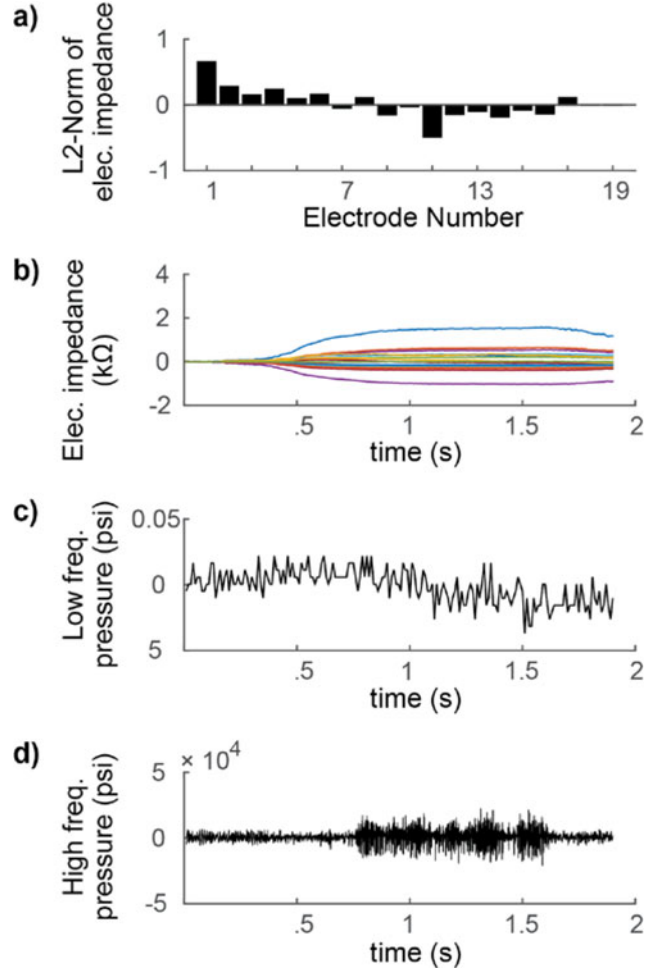
Fig. 6. Representative multimodal tactile data for a single action. a) DNN input vector values are shown as a histogram of the 19 normalized electrode values. Time histories for tactile sensor data for a complete action: b) electrode impedance (100 Hz), c) low frequency fluid pressure (100 Hz), and d) high frequency fluid pressure (2200 Hz).
