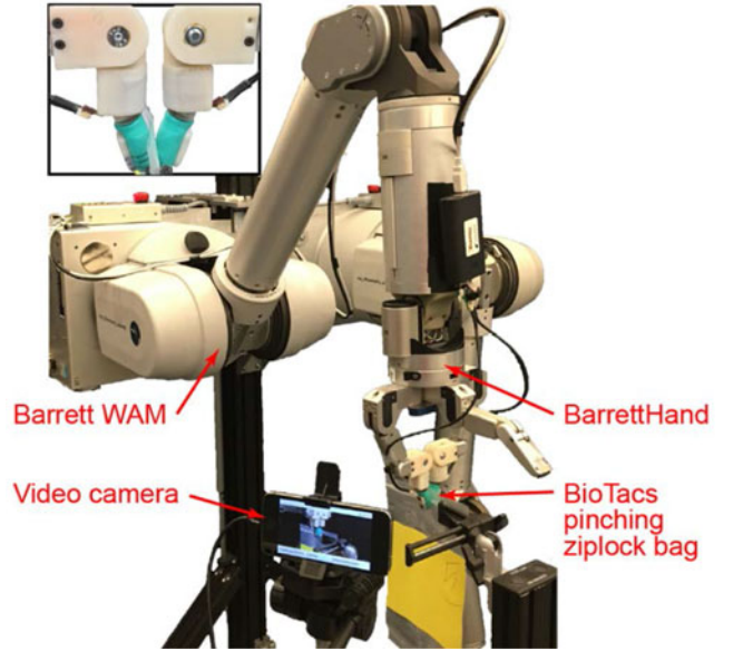
Fig. 1. Experimental set-up used to develop online haptic perception and decision-making capabilities for a functional contour-following task. Inset: A custom adapter enabled a 20 degree contact angle.
